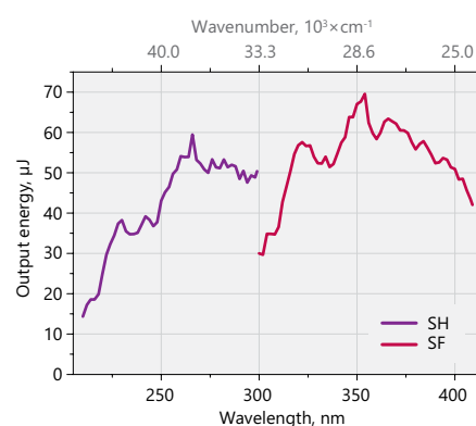
Fig. 2. Typical PT401 tuning curves in SH (210 – 300 nm), SF (300 – 409 nm) ranges
