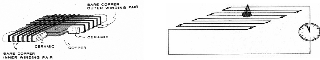
Figure 1.1: Operation principle of the delay-line-anode,
