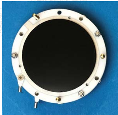
Figure 1.5: If the guide screws are placed in the front ring exactly as in the picture above (MCP contact side facing upwards) it is possible to place the anode/back ring without conflicts of occupied holes. Right: guide pin positions for alternative “bottom up” assembly.
